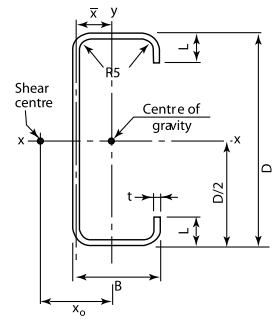
C-Purlin
