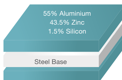
Aluminium-zinc alloy layer (AZ100 coating)
